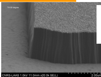
RIE of diamond for power device
