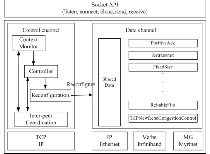
Fig. 2: P2PSAP Protocol architecture
