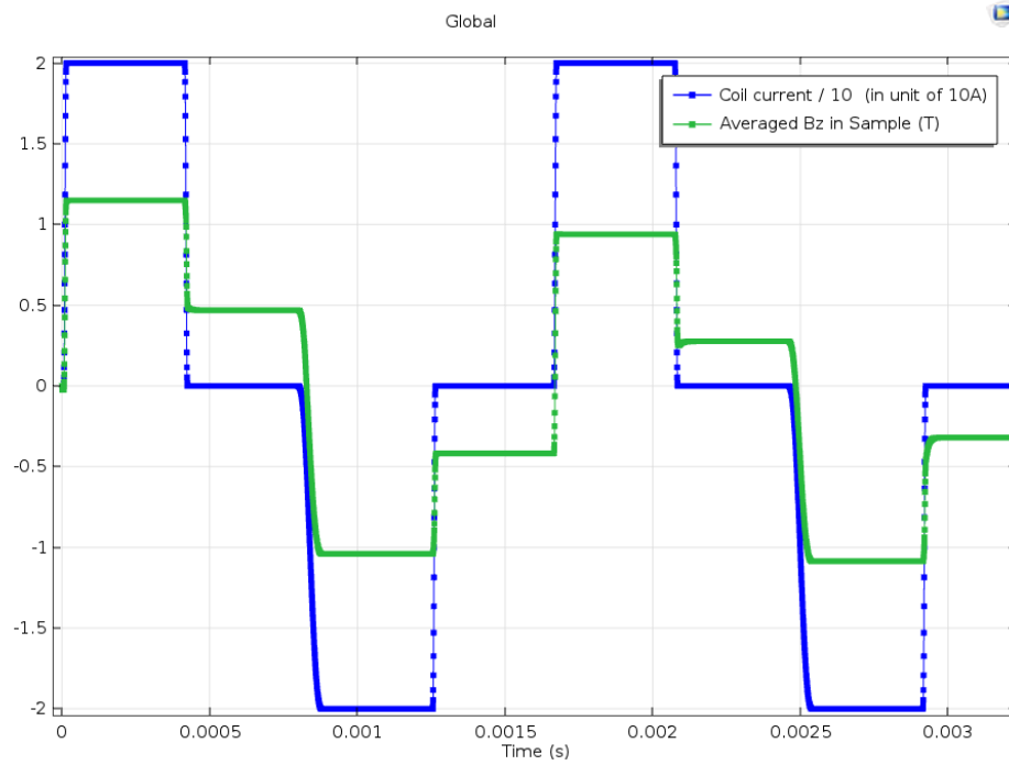
Figure IV-14 Relationship between internal average magnetic field B_z and the coil current intensity I (pulse case, unit is 10A)
