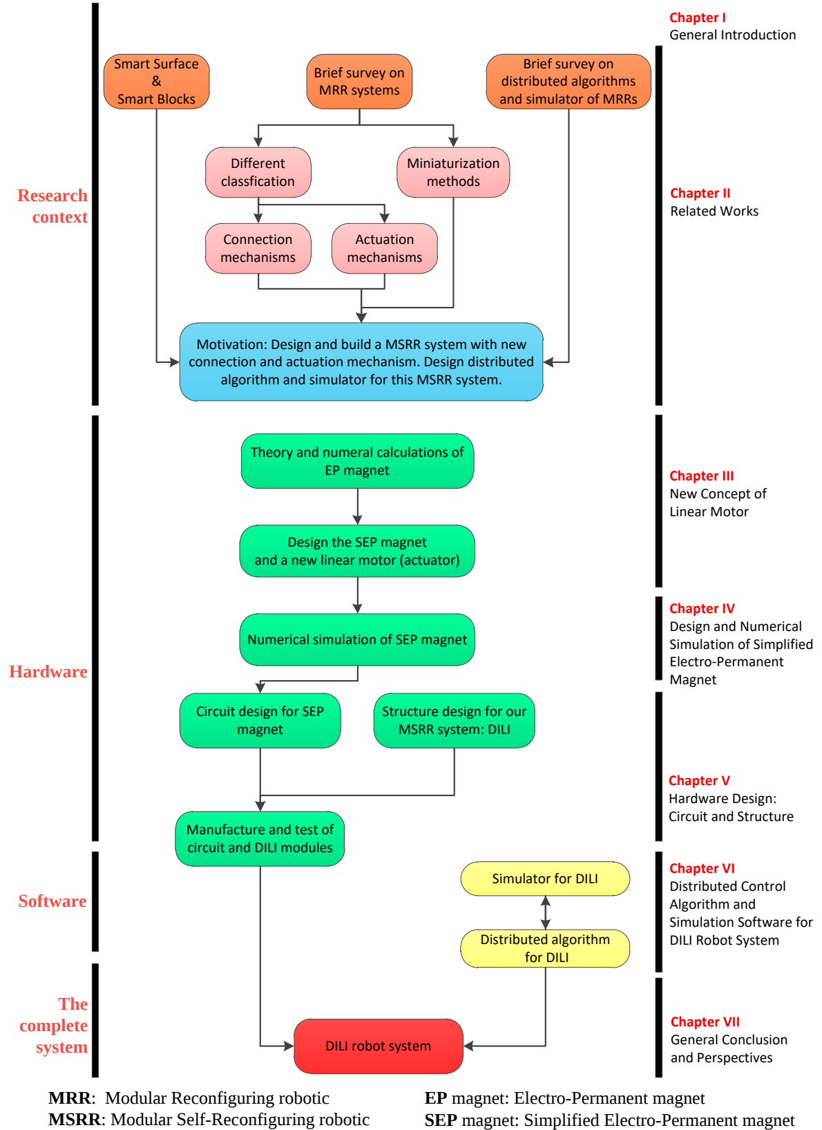
Figure I-1 Thesis structure
