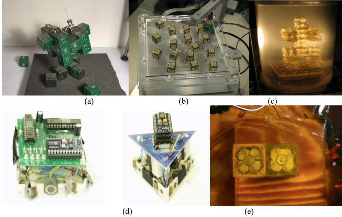
Figure II-8 Some MRRs without actuation system: (a) Miche, (b) Pebbles, (c) Single-material, (d) Two prototype of Stochastic 2D units, (e) Stochastic 3D
