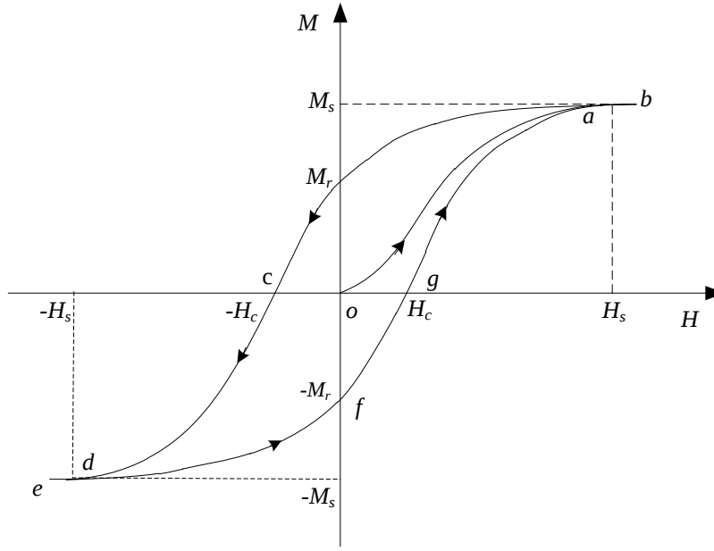
Figure IV-1 Hysteresis loop
