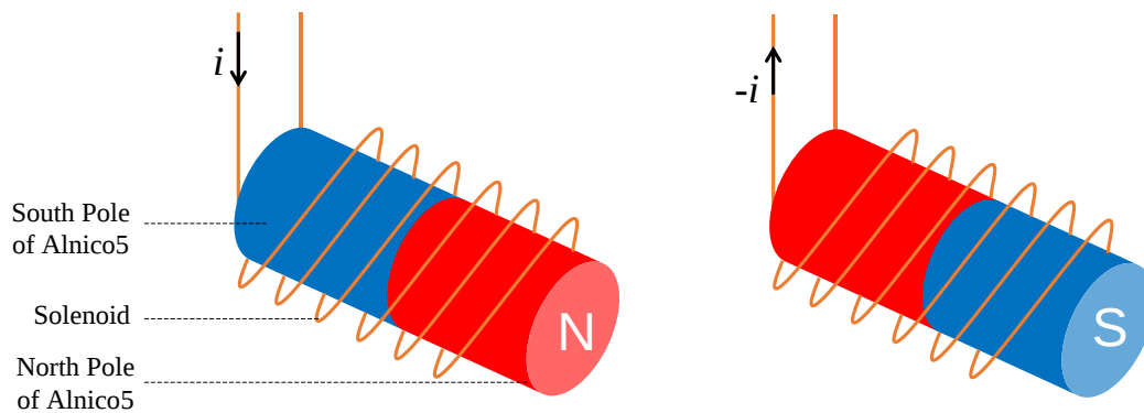
Figure III-5 The principle of SEP
