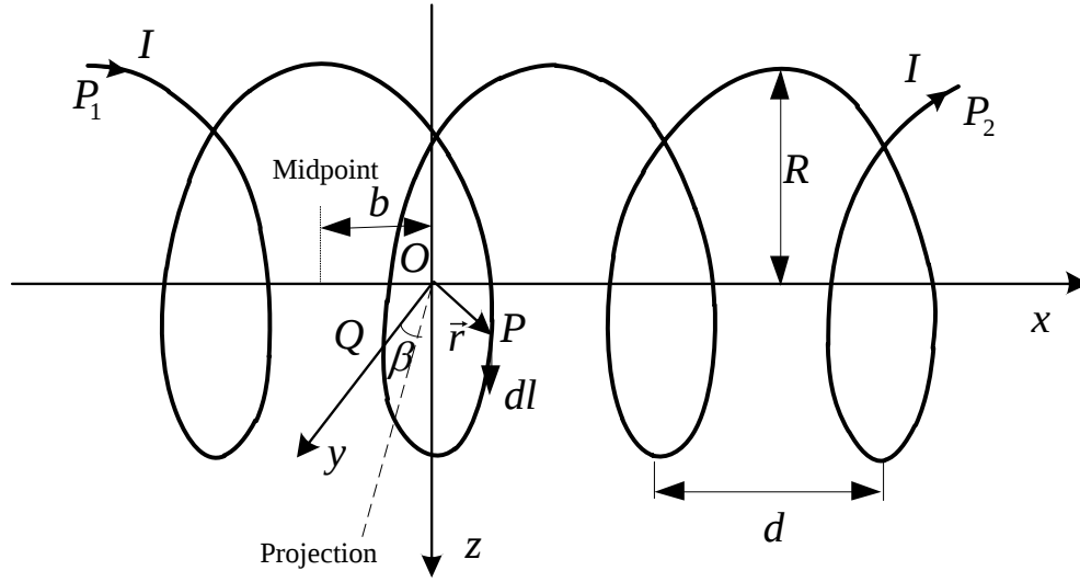
Figure III-4 Structure of solenoid
