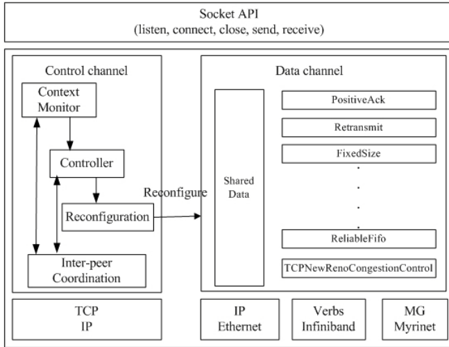
Figure 1. P2PSAP Protocol architecture
