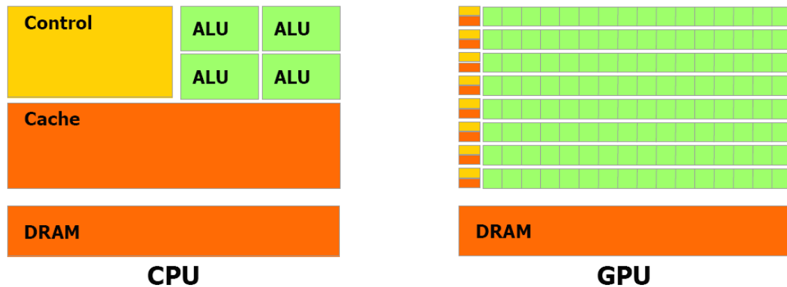
FIGURE IV.2 – Architecture CPU et architecture GPU (NVIDIA).
